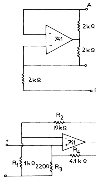
FIG. 2. Laboratory realization of (a) the negative conductance G and (b) the nonlinear resistor R_N .
